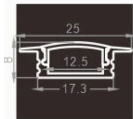
Installation Diagram
